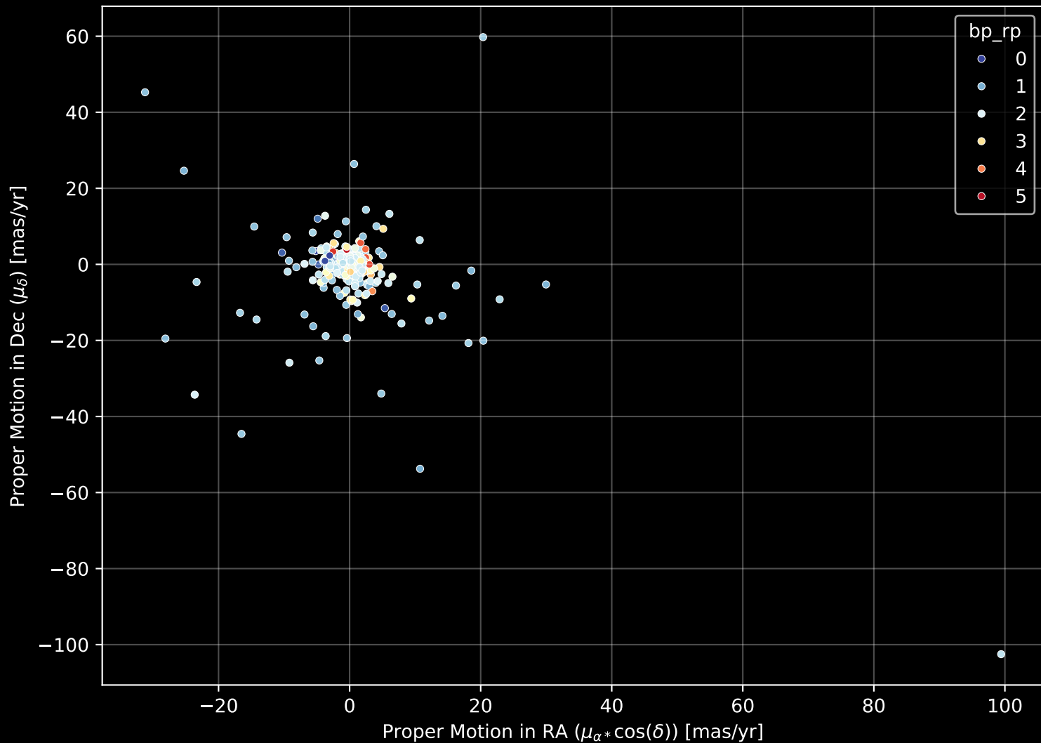
APOGEE DR17 Field: [214-12] Proper Motion Diagram (n= 375)
