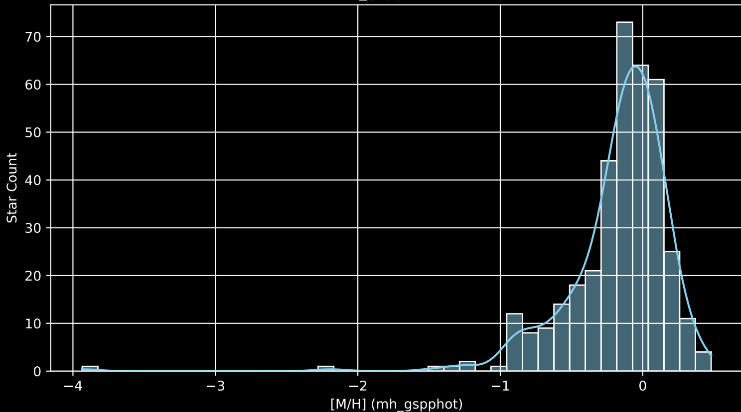
APOGEE DR17 Field: [214-12 [M/H] (mh_gspphot) (n= 371)
