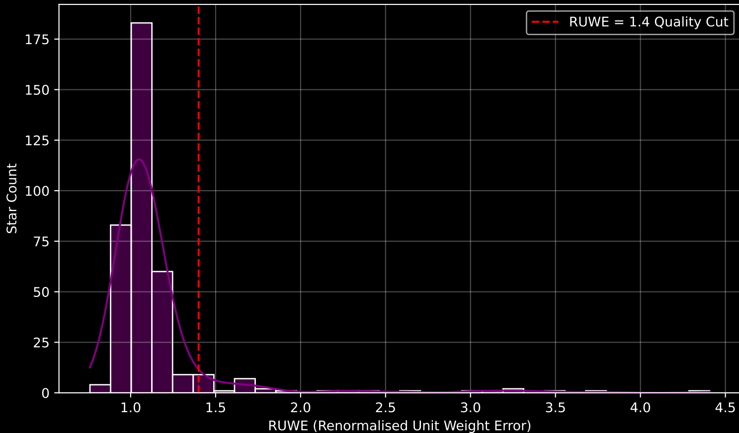
GAPOGEE DR17 Field [214-12] RUWE Distribution (n= 370)
