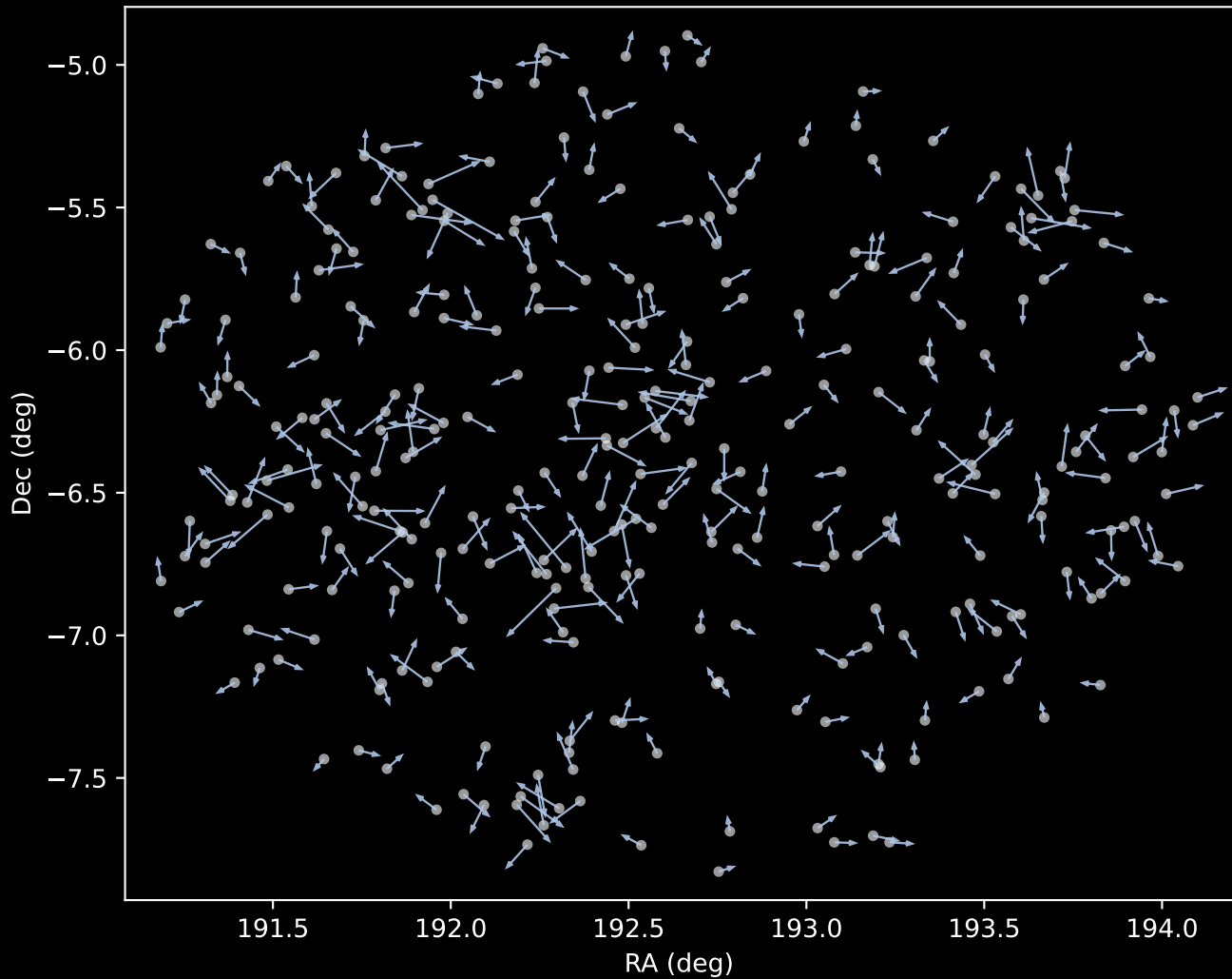
APOGEE DR17 Cluster 1 Proper Motion Vectors (n=310)
