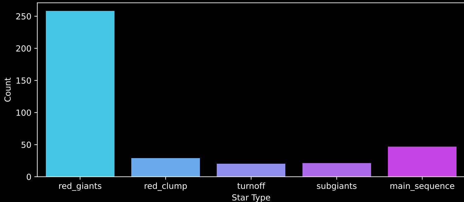
APOGEE DR17 Field: [214-12] Count plot of Star Type
