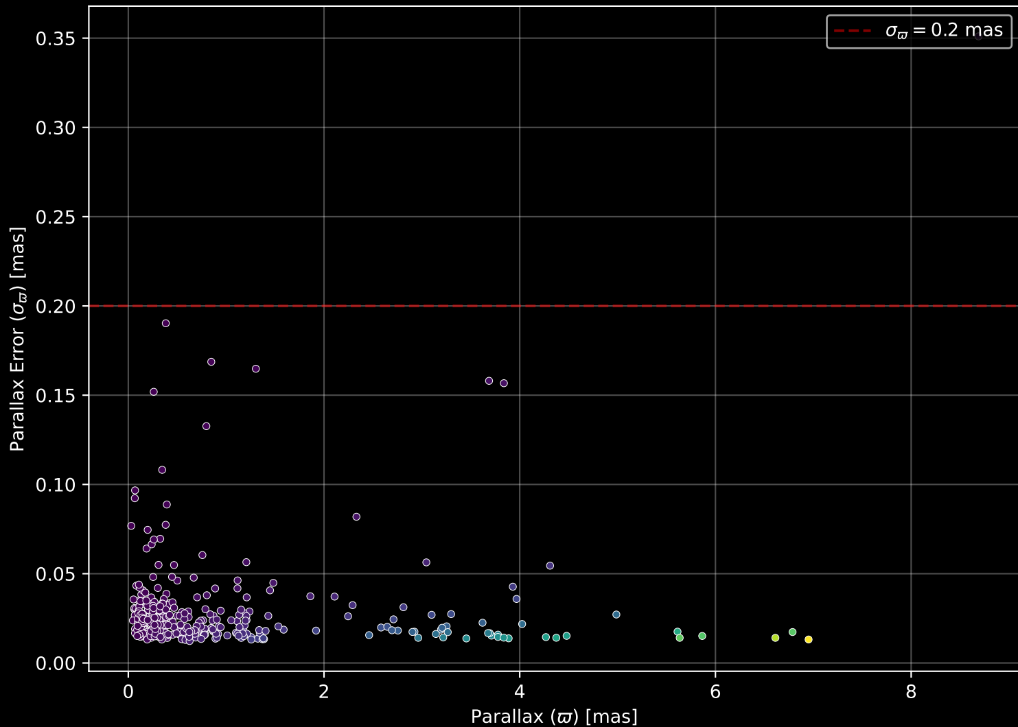
APOGEE DR17 Field: [214-12] Parallax Quality (n= 375)
