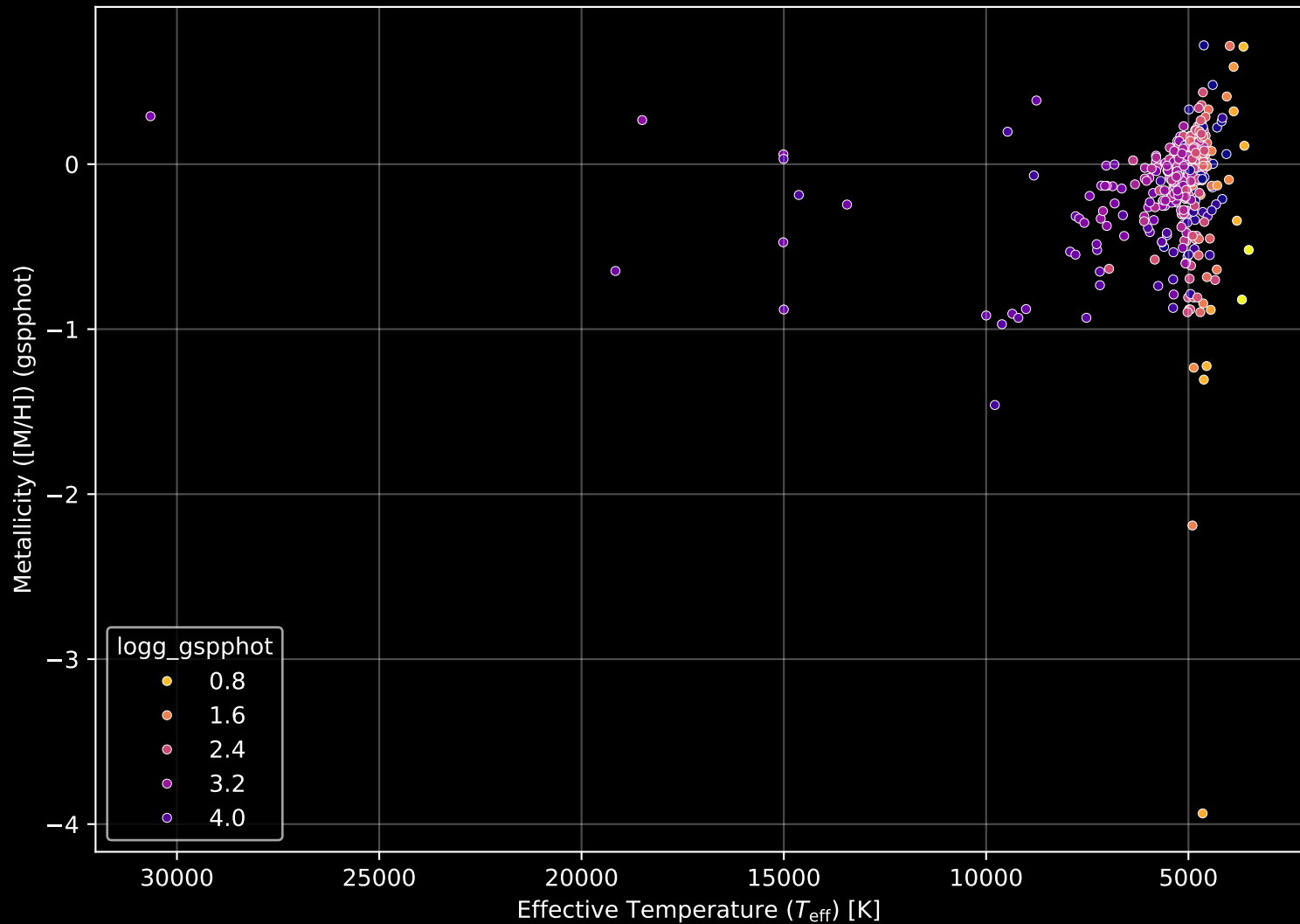
APOGEE DR17 Field: [214-12] Stellar Population Parameters (n= 375)
