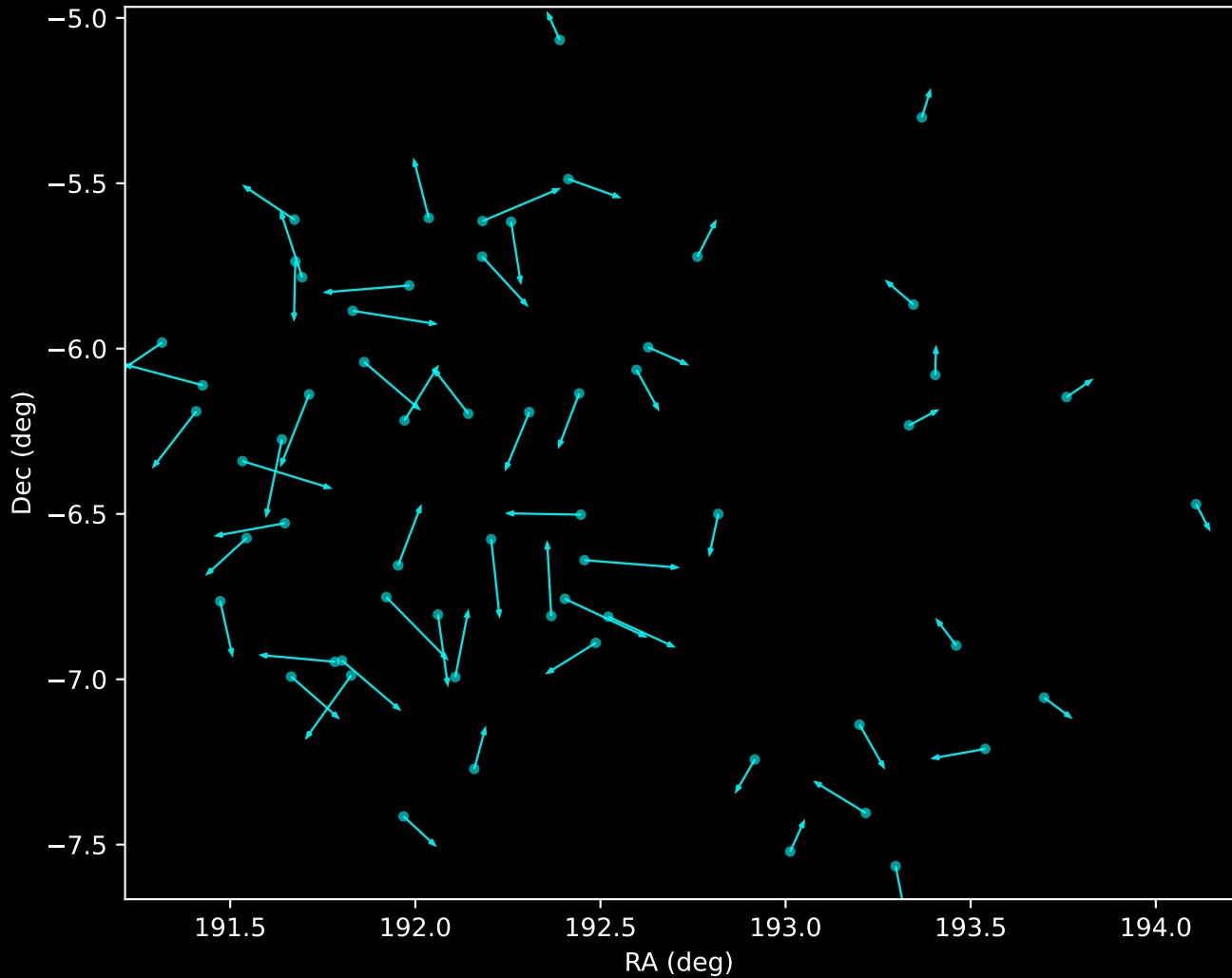
APOGEE DR17 Noise Stream Proper Motion Vectors (n=60)
